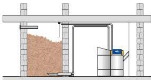
3 Fuel transport with suction lance
